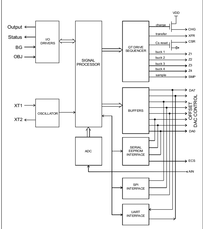
FIGURE 1-1 BLOCK DIAGRAM
