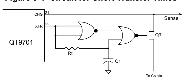
Figure 3-1 Circuit for Short Transfer Times
