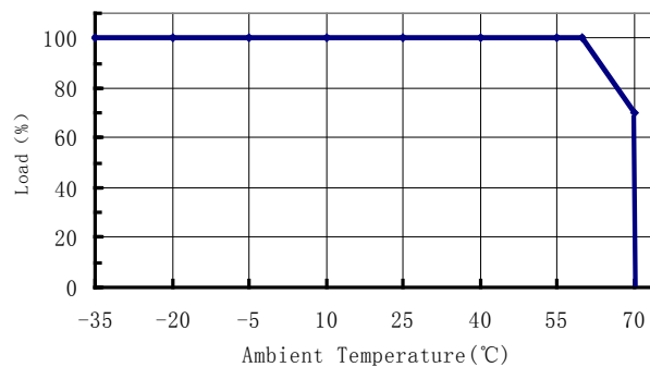
Ambient Temperature vs. Load
