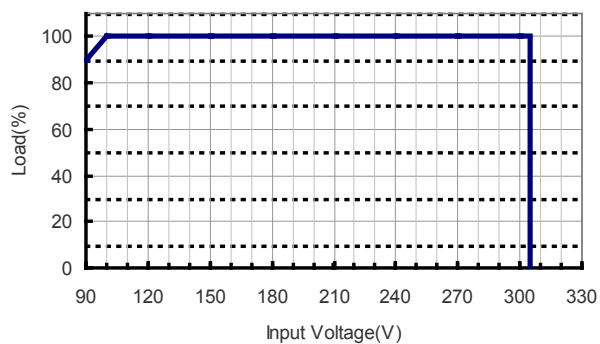
Derating Curve
