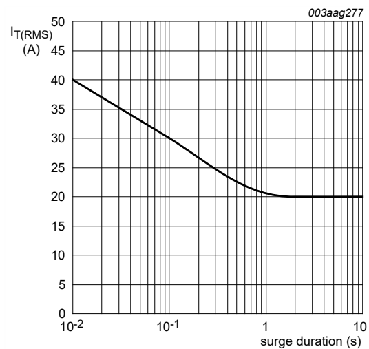
Fig. 3. RMS on-state current as a function of surge duration; maximum values f = 50 \text{ Hz}; T_{mb} = 103 \text{ °C}
