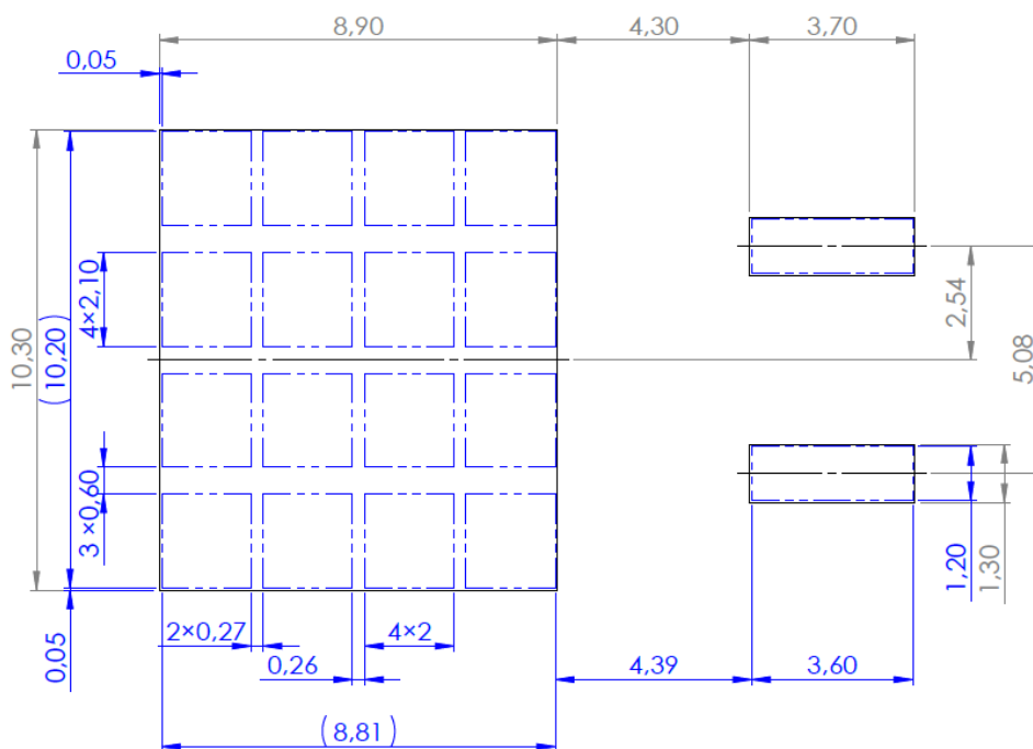
Figure 11. D 2 PAK stencil definitions (dimensions are in mm)
