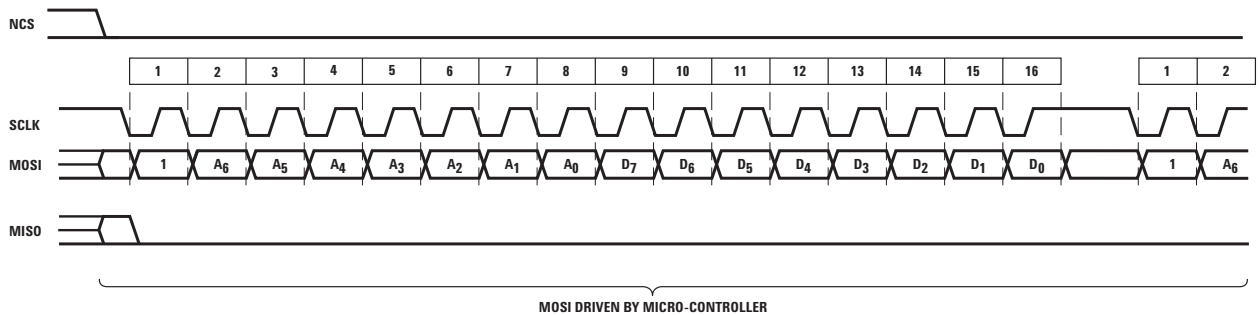
Figure14. Write operation.
