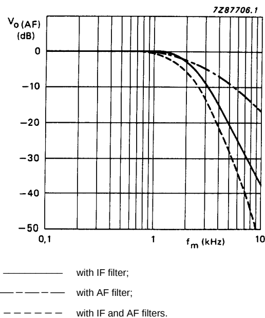
Fig.7 Typical frequency response curves from Fig.1 showing the effect of filtering.
