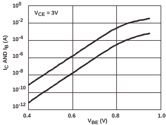
FIGURE 3. GUMMEL PLOT
