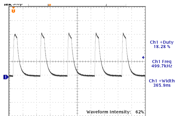
500 KHz Frequency, 125 A Output
