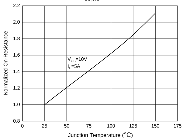
Fig. 4 - R_{DS(ON)} —Temperature
