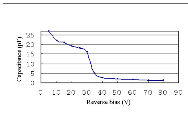
Fig. 4 Typical APD Capacitance
