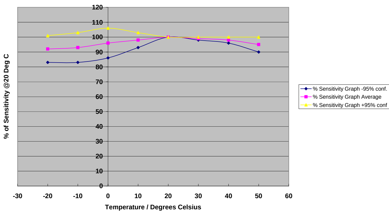
EC4-200-Cl2 Graph of Net Sensitivity vs Temperature
