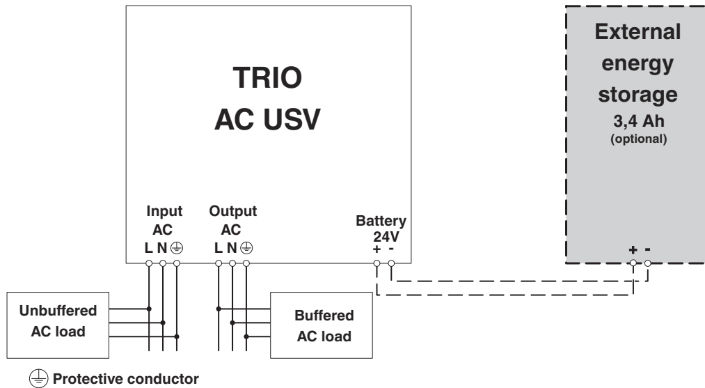
Figure 10 Schematic design
