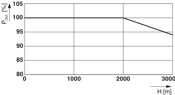
Figure 26 Altitude-dependent derating
