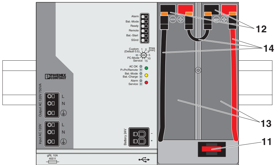
Figure 2 Position of the function elements (part 2)
