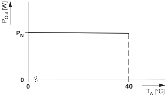
Figure 25 Temperature-dependent derating
