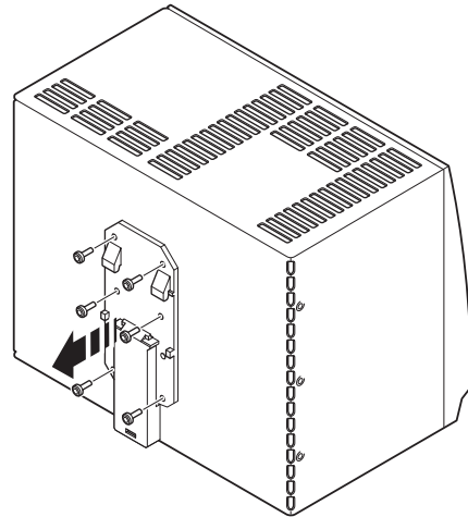
Figure 8 Disassembling the universal DIN rail adapter
