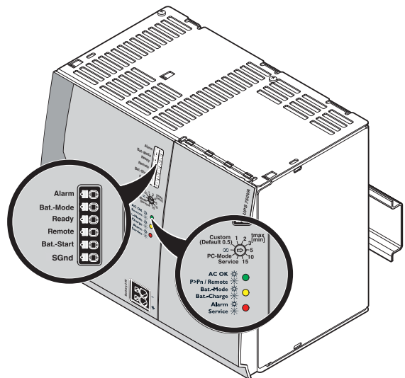
Figure 21 LED indicators and signal outputs
