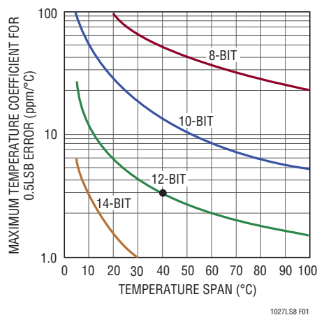
Figure 1. Maximum Allowable Reference Drift
