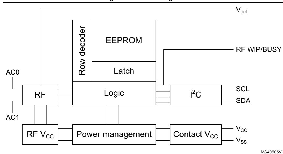
Figure 5. Circuit diagram
