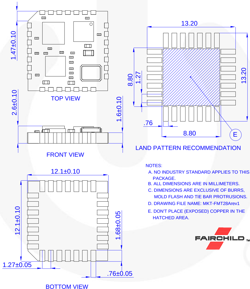
Figure 17. FMT28_028 Package
