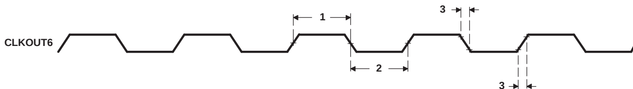
Figure 5-15. CLKOUT6 Timing
