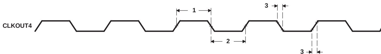
Figure 5-14. CLKOUT4 Timing
