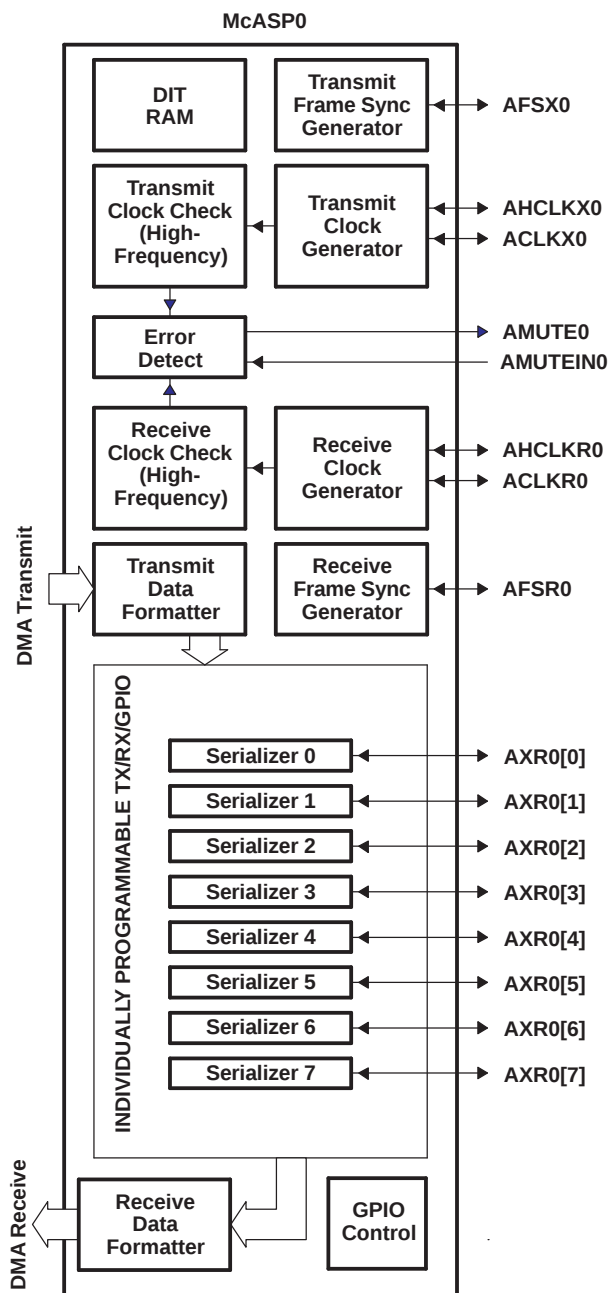
Figure 5-34. McASP0 Configuration
