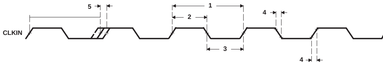
Figure 5-13. CLKIN Timing
