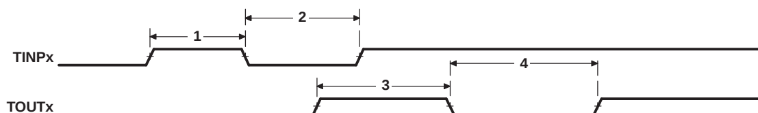
Figure 5-65. Timer Timing
