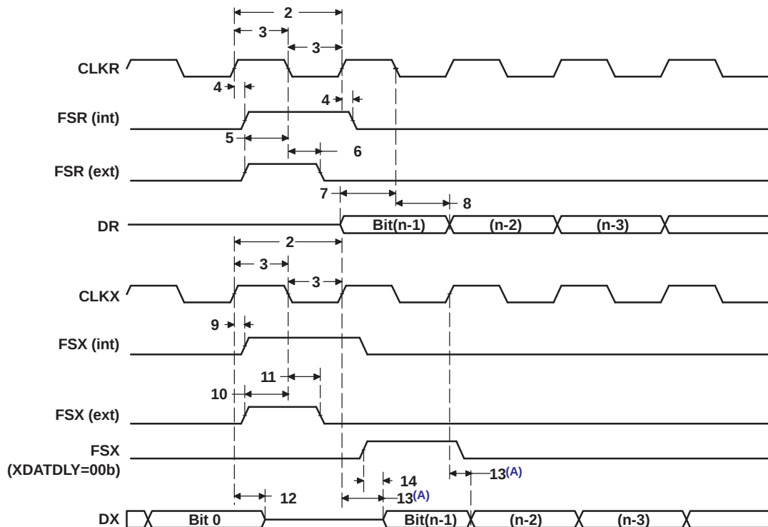
Figure 5-48. McBSP Timing
