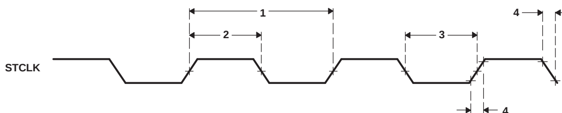
Figure 5-58. STCLK Timing
