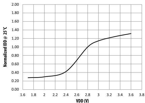
Figure 8 Normalized Standby IDD vs. VDD
