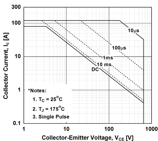
Figure 16. SOA Characteristics
