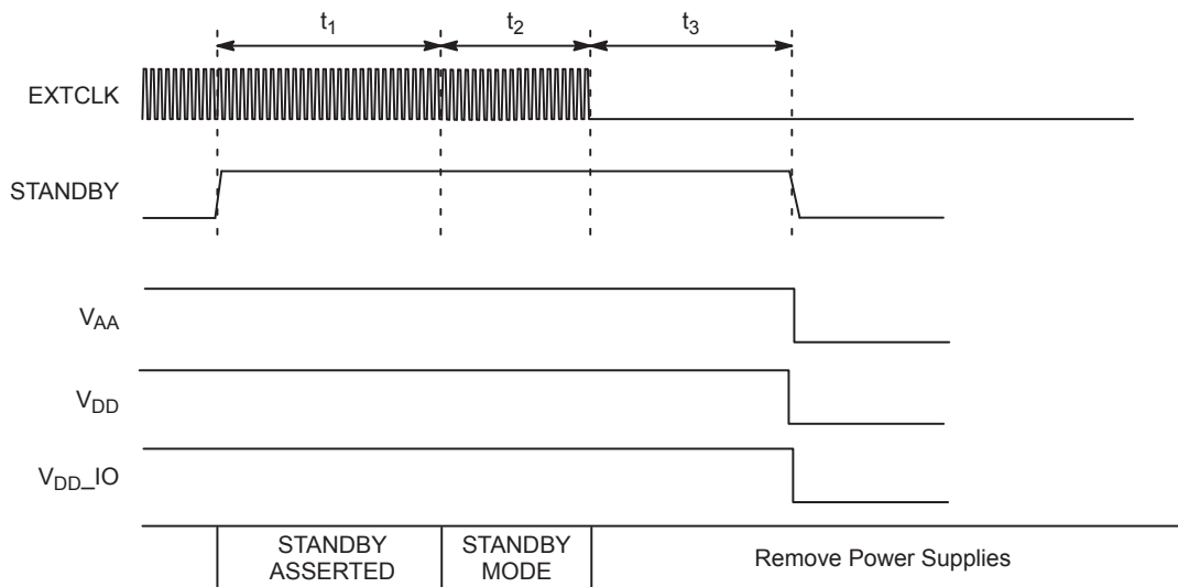
Figure 30. Recommended Power Down Sequence
