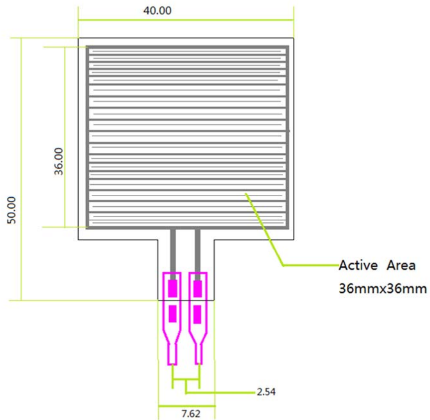
RP-S40-ST Dimension Diagram
