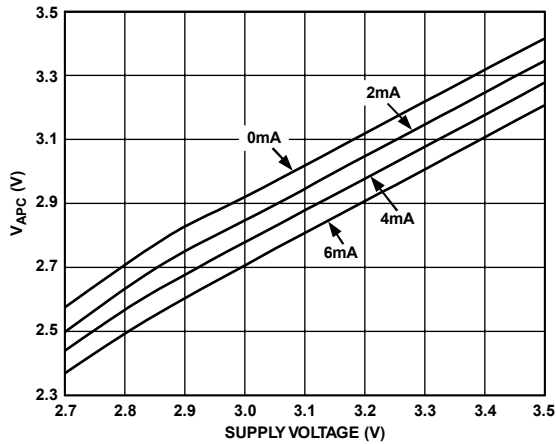
Figure 21. Maximum V_{APC} Voltage vs. Supply Voltage by Load Current
