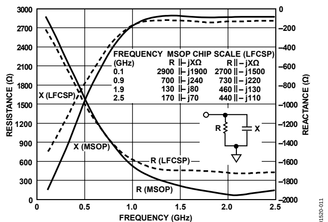
Figure 11. Input Impedance
