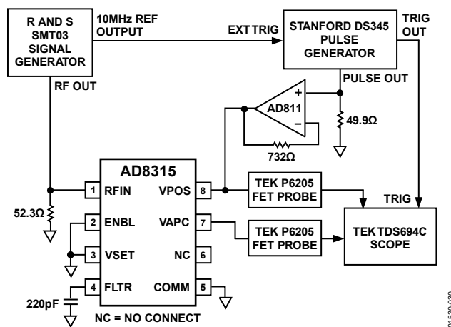
Figure 30. Test Setup for Power-On and Power-Off Response with VSET and ENBL Grounded
