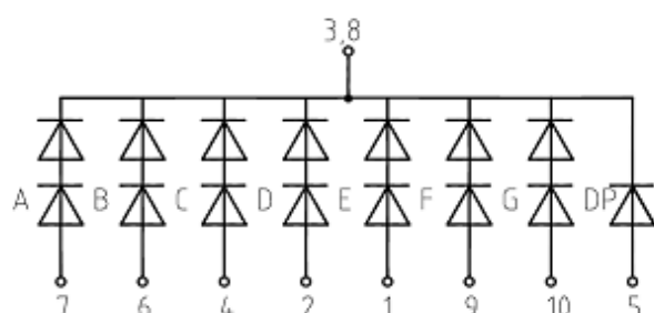
Common Cathode
