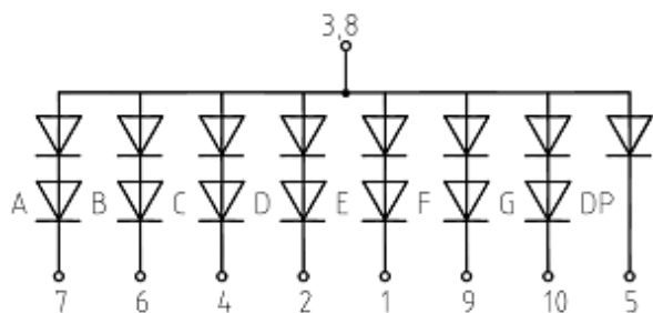
Common Anode
