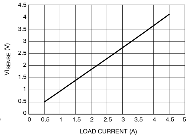
Figure 8. V_{I\text{SENSE}} vs. Load Current
