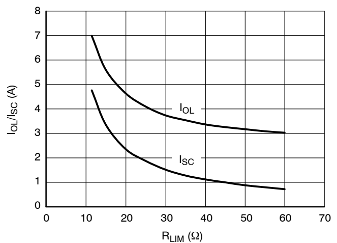
Figure 12. I_{OL} and I_{SC} vs. R_{LIM}
