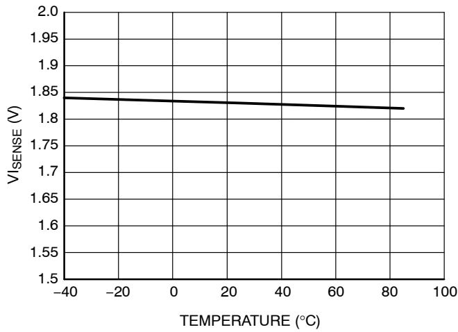
Figure 7. V_{I\text{SENSE}} vs. Temperature
