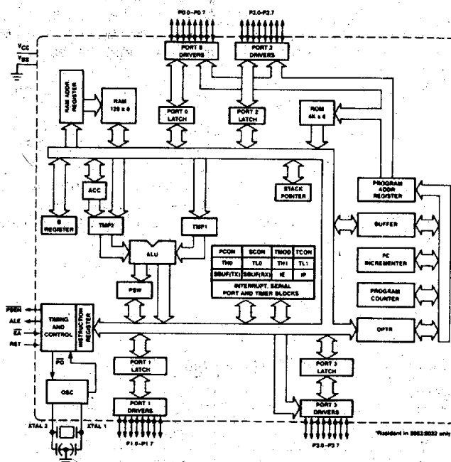
Figure 1. Block Diagram
