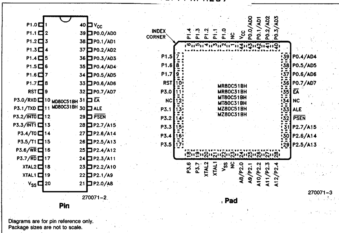
Figure 2. Connection Diagram
