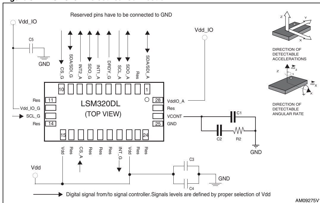
Figure 5. LSM320DL electrical connection
