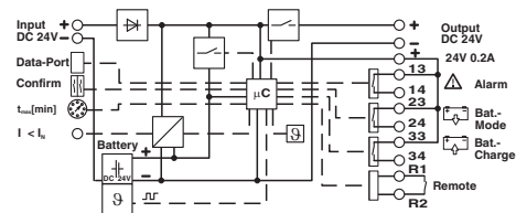
Block diagram
