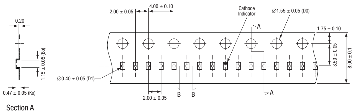
Figure 15. SOD-882 Package Dimension Drawing
