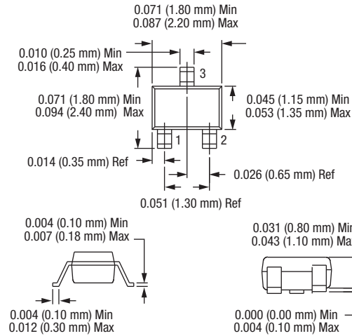
Figure 5. SC-70 Package Dimension Drawing
