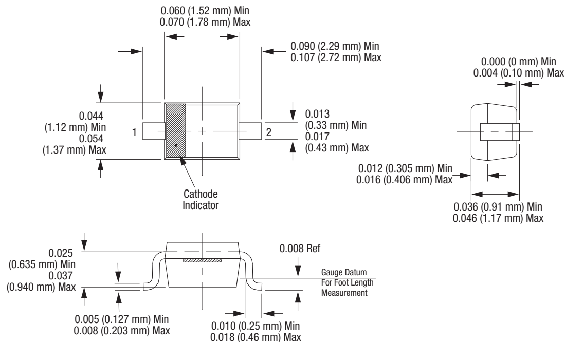
Figure 11. SOD-323 Package Dimension Drawing
