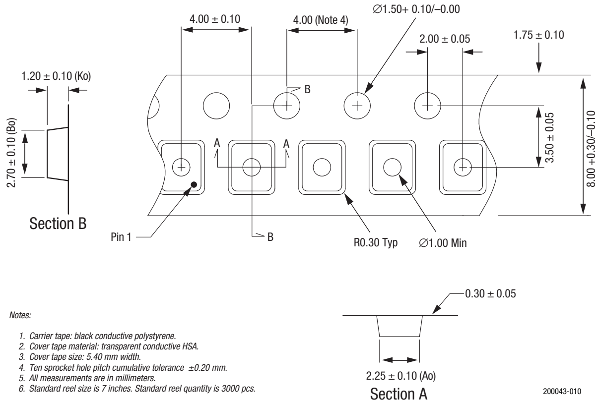
Figure 10. SC-88 Tape and Reel Dimensions
