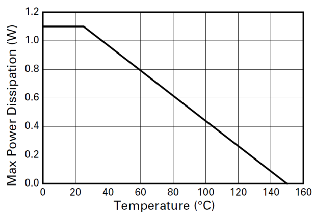
Derating Curve
