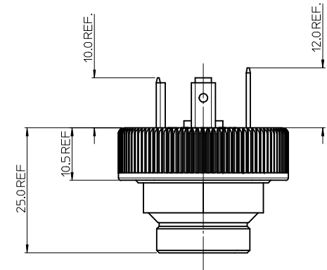
VERSION A (PG9, PG11 OR PG13.5 THREAD)
