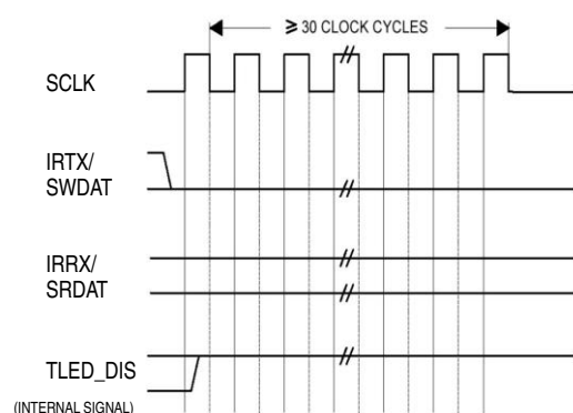
Figure 7. Initial Reset Timing
