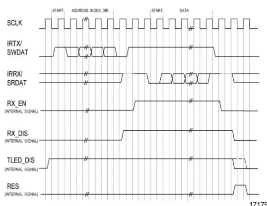
Figure 11. Read Data Waveform
