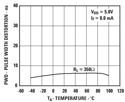
Figure 15. Typical pulse width distortion vs. temperature for 5V operation.
