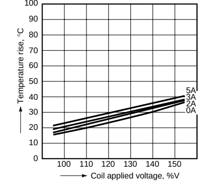
3.-(1) Coil temperature rise (180 mW) Tested sample: PA1a-24V Measured portion: Inside the coil Ambient temperature: 20°C 68°F
