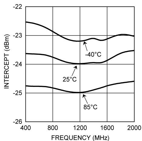
Logarithmic Intercept vs. Frequency (LMV228 in LLP)
