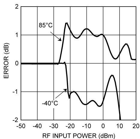
Output Variation vs. RF Input Power Normalized to 25^\circ C @ 1900 MHz (LMV228 in LLP)
