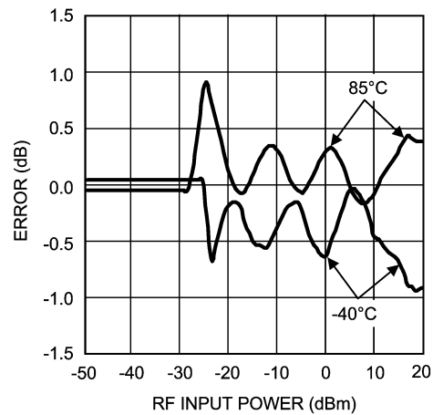
Output Variation vs. RF Input Power Normalized to 25^\circ C @ 2000 MHz (LMV228 in microSMD)
