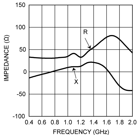
RF Input Impedance vs. Frequency @ Resistance and Reactance (LMV225 in LLP)
