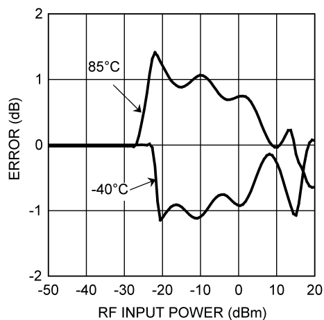
Output Variation vs. RF Input Power Normalized to 25^\circ C @ 900 MHz (LMV228 in LLP)
