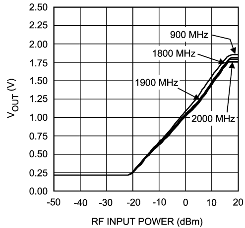
Output Voltage vs. RF Input Power (LMV226)
