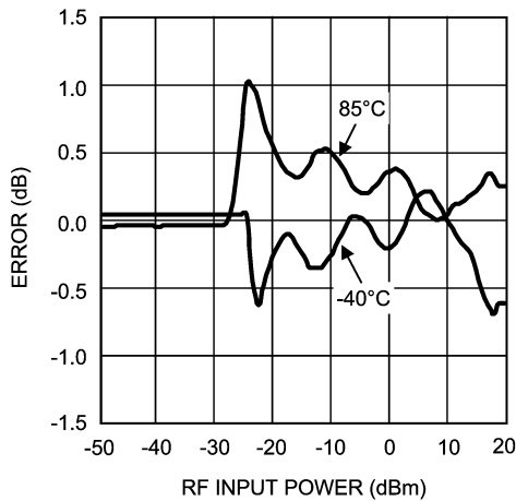
Output Variation vs. RF Input Power Normalized to 25^\circ C @ 900 MHz (LMV228 in microSMD)
