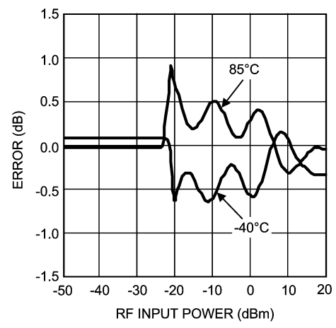
Output Variation vs. RF Input Power Normalized to 25°C @ 2000 MHz (LMV226)
