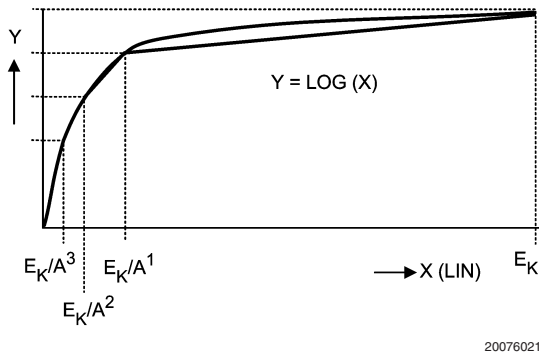
FIGURE 9. Log-Function on Lin Scale
