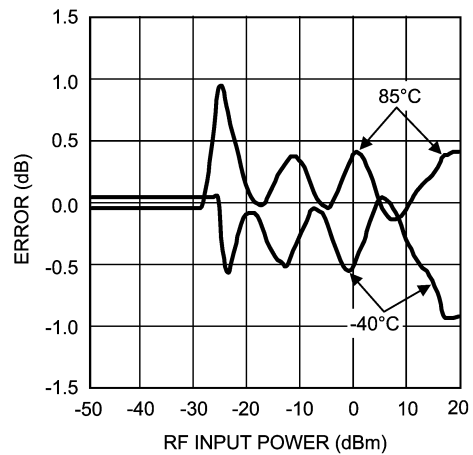
Output Variation vs. RF Input Power Normalized to 25^\circ C @ 1900 MHz (LMV228 in microSMD)
