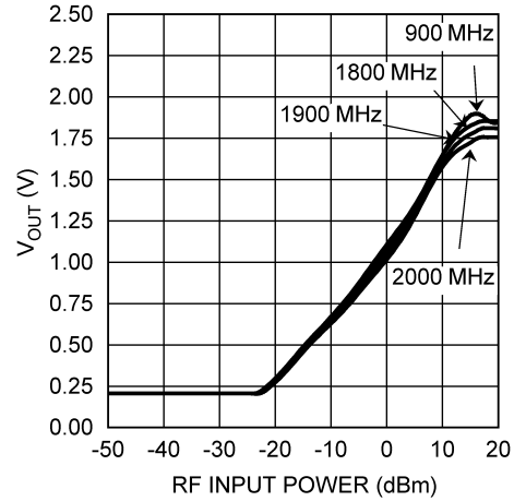
Output Voltage vs. RF Input Power (LMV228 in LLP)
