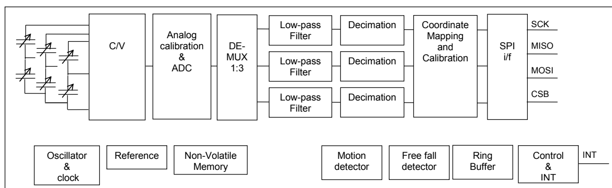
Figure 1 SCA3000-E04 Block Diagram
