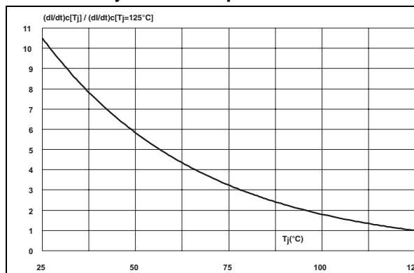
Figure 12. Relative variation of critical rate of decrease of main current vs. junction temperature
