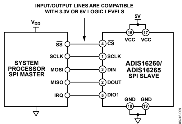
Figure 9. Electrical Connection Diagram
