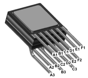
Figure 4. Pin Configuration (3D View)
