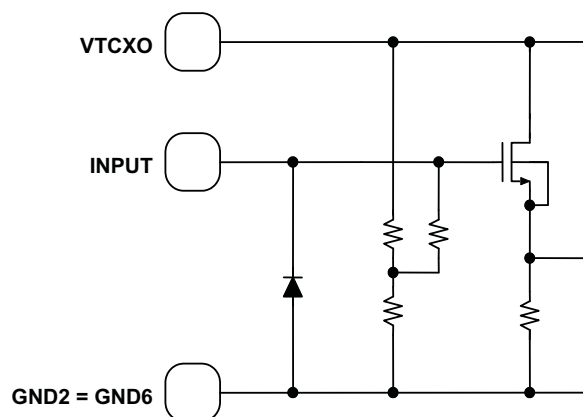
Figure 59. SYSCLK_IN
