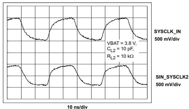
CLOCK DISTRIBUTION/SIN_SYSCLK2 INPUT vs OUTPUT (-1 dB TYP)
