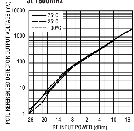
LTC4400-2 Detector Characteristics at 1800MHz
