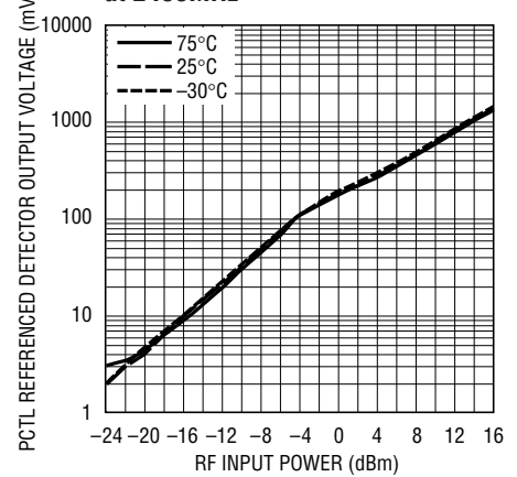
LTC4400-1 Detector Characteristics at 2400MHz
