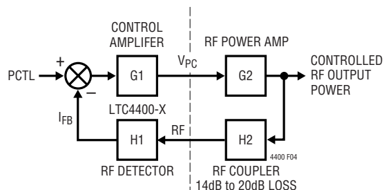
Figure 4. Closed-Loop Block Diagram
