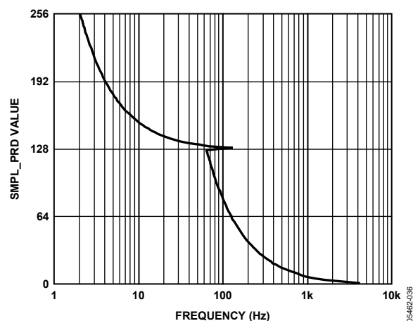
Figure 33. SMPL_PRD Values vs. Sample Frequency
