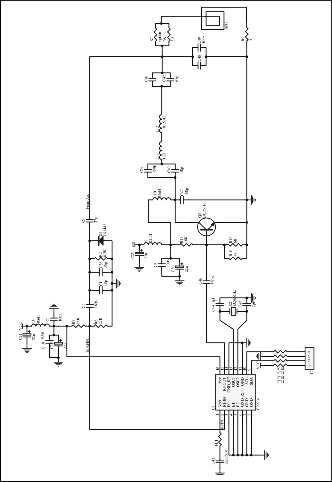
Figure 2. Schematic 2/2
