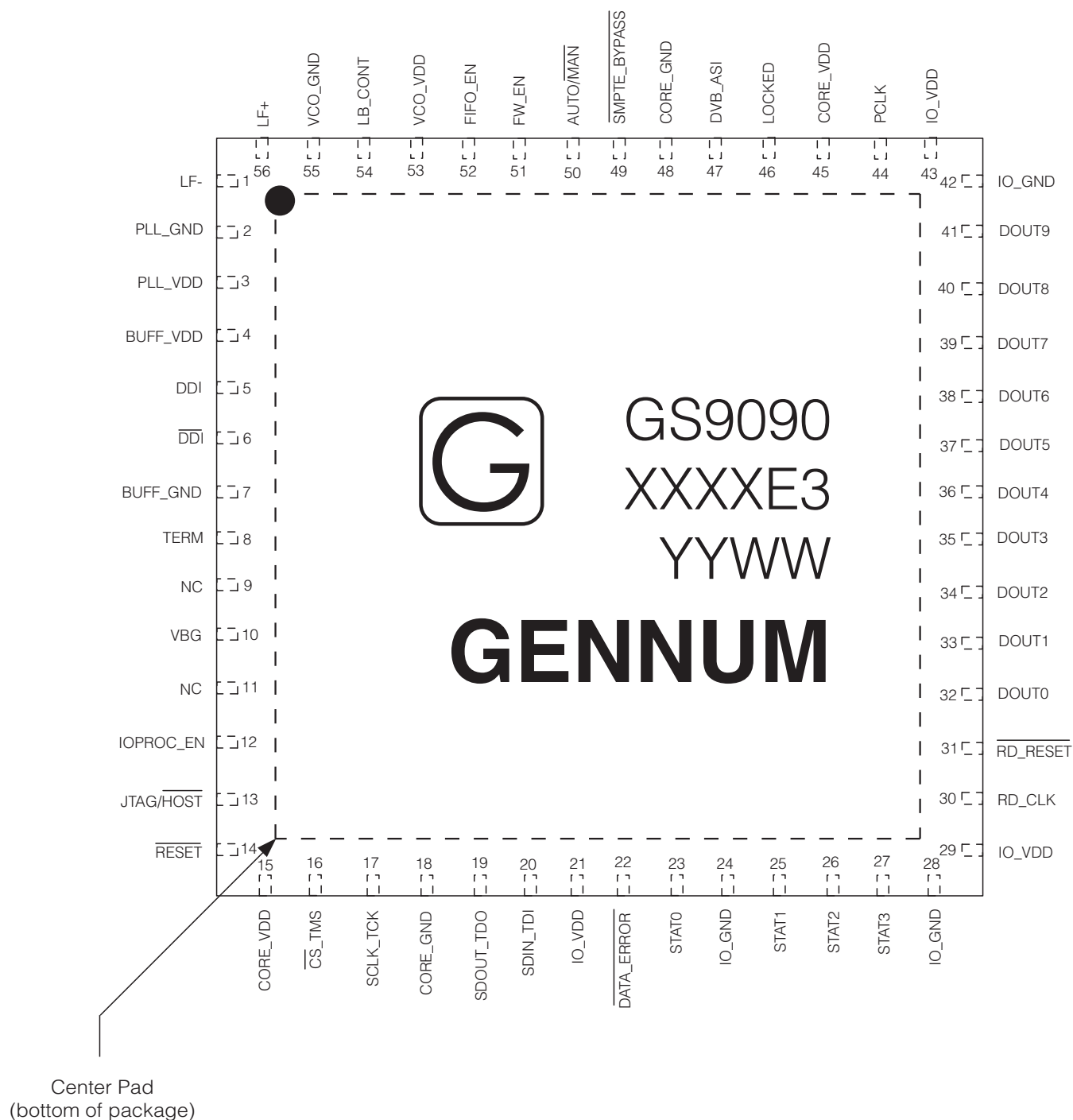
Figure 1-1: Pin Assignment
