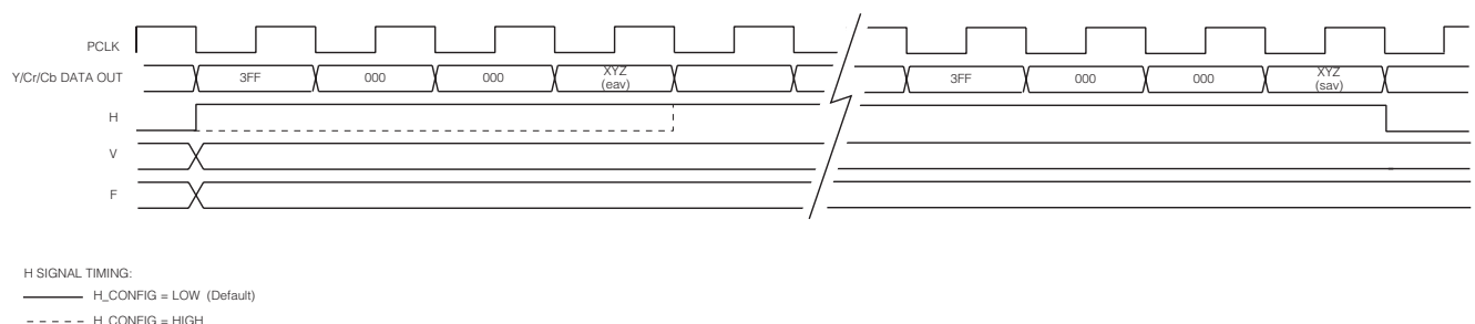
Figure 3-3: H,V,F Timing
