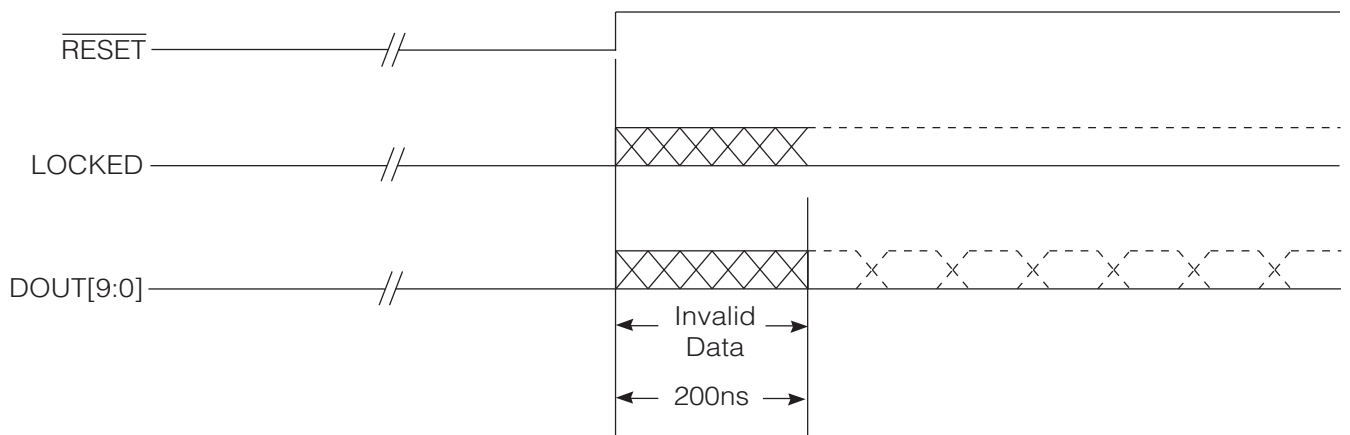
Figure 3-20: Reset Timing
