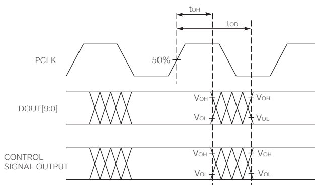
Figure 3-13: PCLK to Data & Control Signal Output Timing
