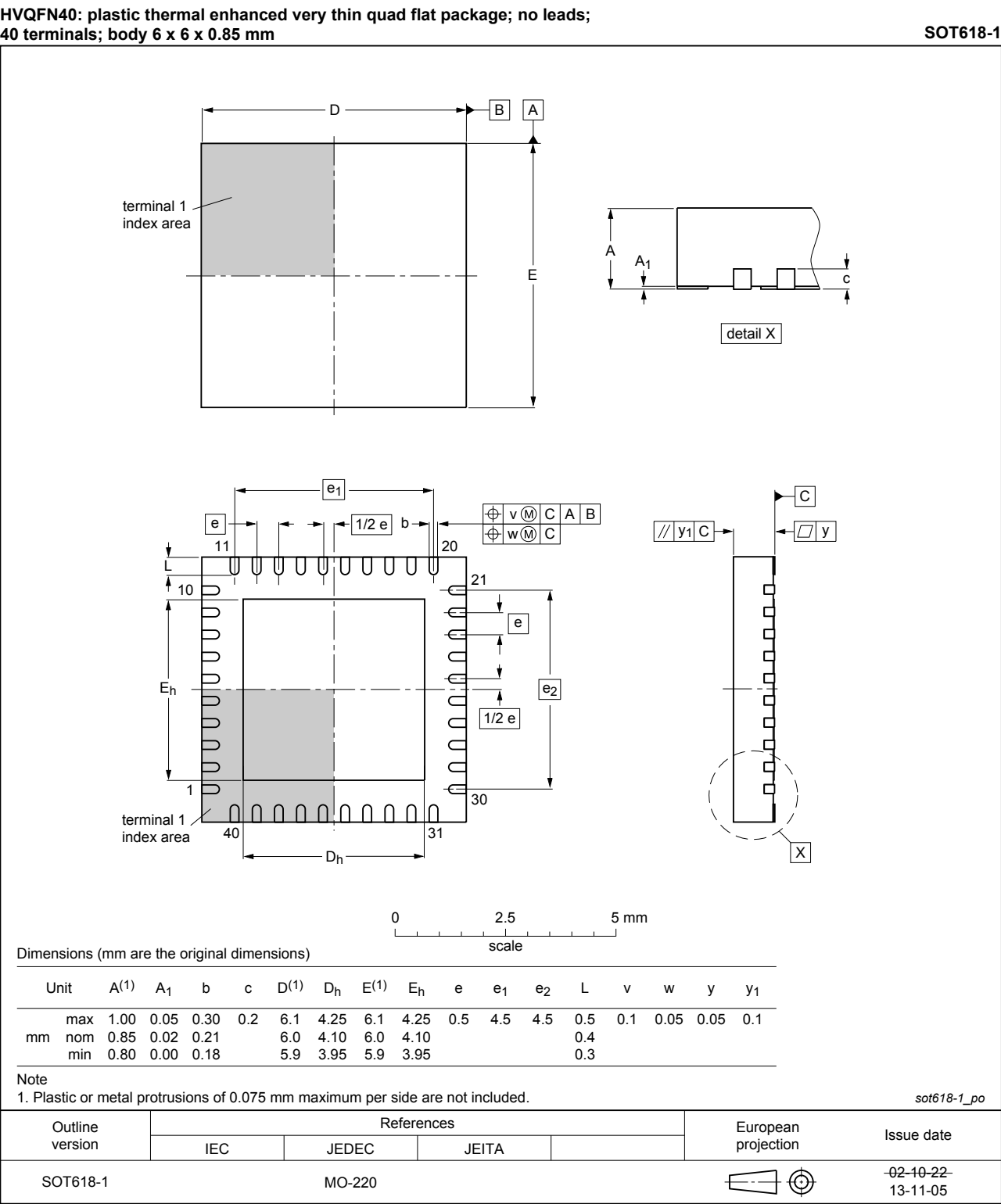
Figure 49. Package outline SOT618-1
