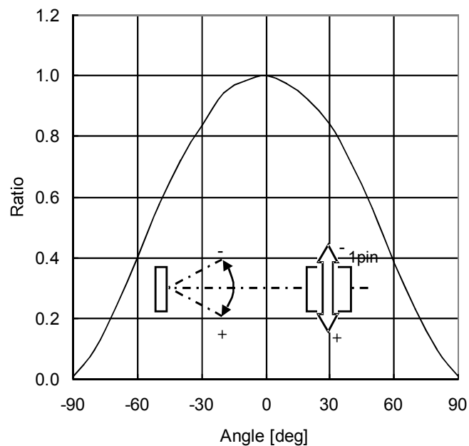
Figure 4. Directional Characteristics 2
