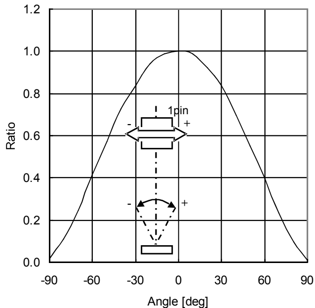
Figure 3. Directional Characteristics 1
