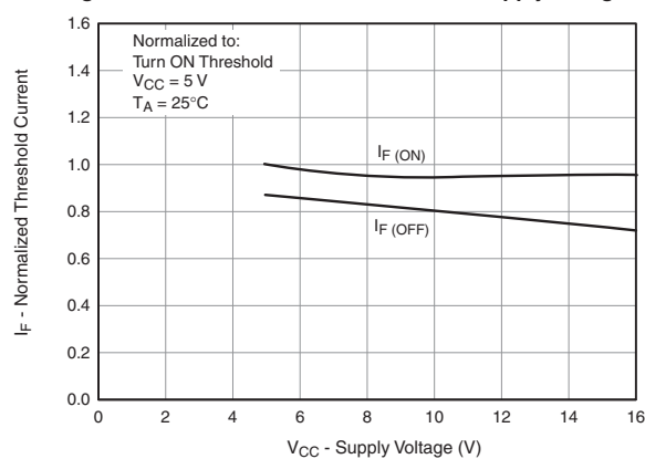
Fig. 4 Normalized Threshold Current vs. Supply Voltage
