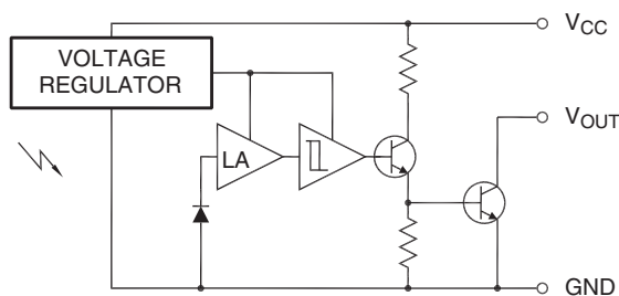
QSE159 Open-Collector Output Inverter
