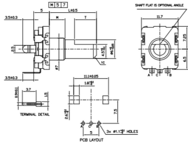
MODEL EN11-VNM (Side Adjust, without Switch, Threaded Bushing)
