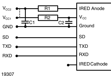
Fig. 3 - Recommended Application Circuit
