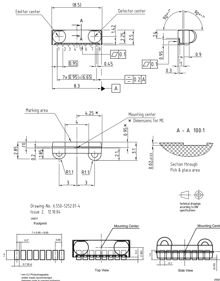
Fig. 8 - Package Drawing
