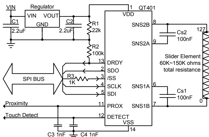
Figure 1-1 QT401 Wiring Diagram
