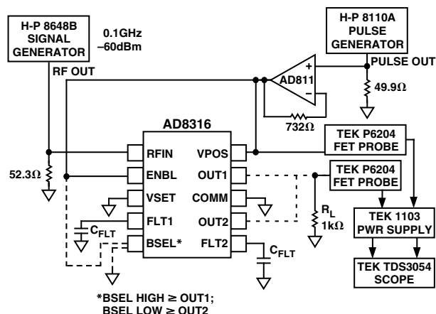
TPC 27. Test Setup for Power-On and Power-Off Response with VSET Grounded
