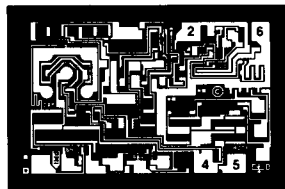
DIE SIZE 0.074 \times 0.048 inch, 3552 sq. mils ( 1.88 \times 1.22 mm, 2.29 sq. mm)
